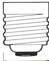
39.5 max. E40 (GES) Goliath Edison Screw
