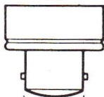
22 max. BY22d Sodium Bayonet Cap
