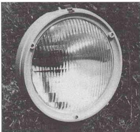
HIGH INTENSITY UNIDIRECTIONAL APPROACH LIGHT
